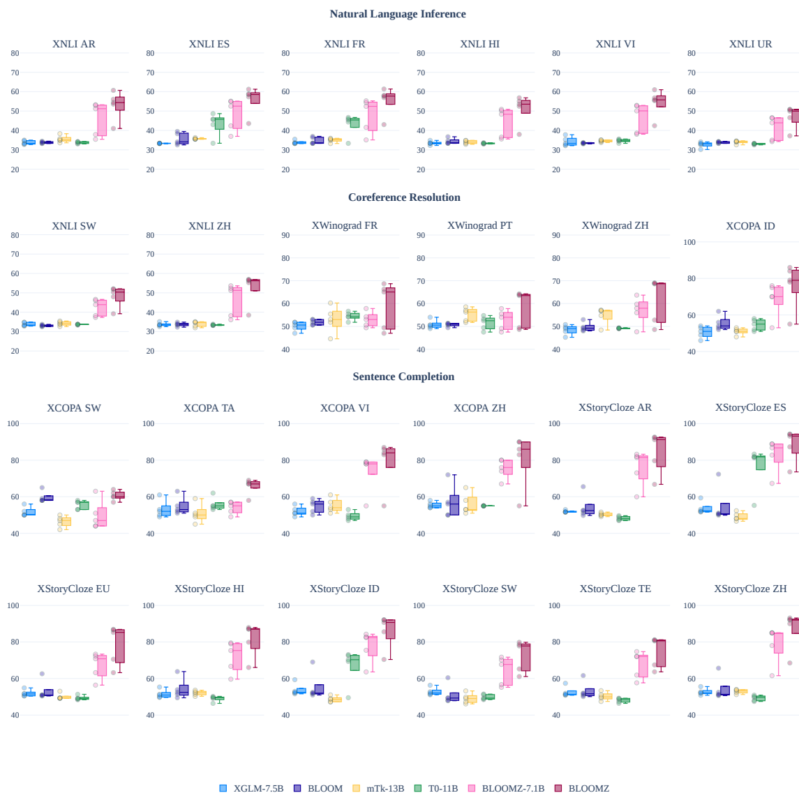
Figure 10: BLOOMZ zero-shot task generalization. Five untuned prompts are evaluated for each dataset and plotted. T0 is monolingual (English) while other models are multilingual. T0 performance may be hurt by its inability to tokenize some non-English texts.
