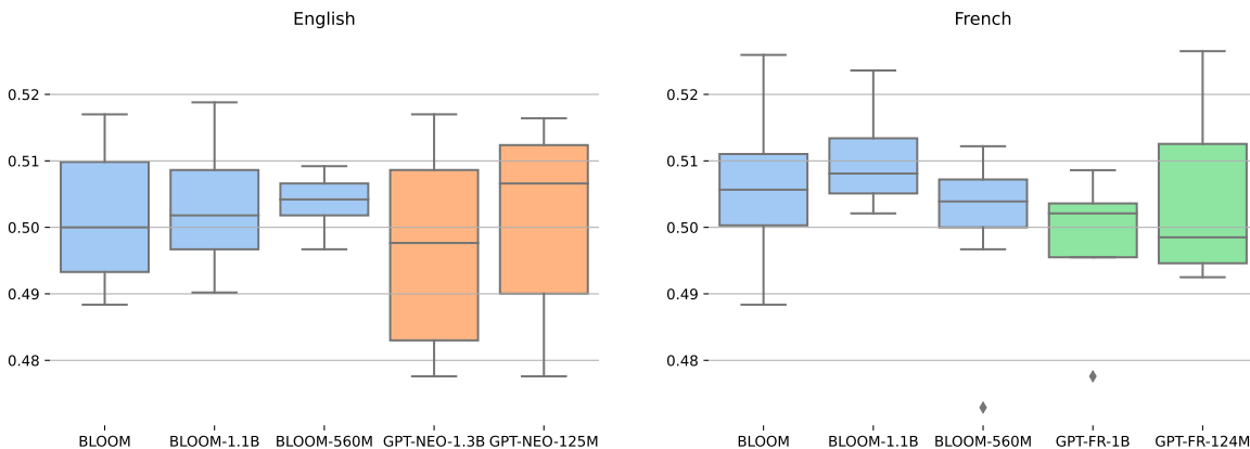
Figure 12: Overall accuracy of BLOOM on crowS-Pairs per prompt for English and French. Results on the two smallest BLOOM models and monolingual GPT models of comparable size are also shown.
